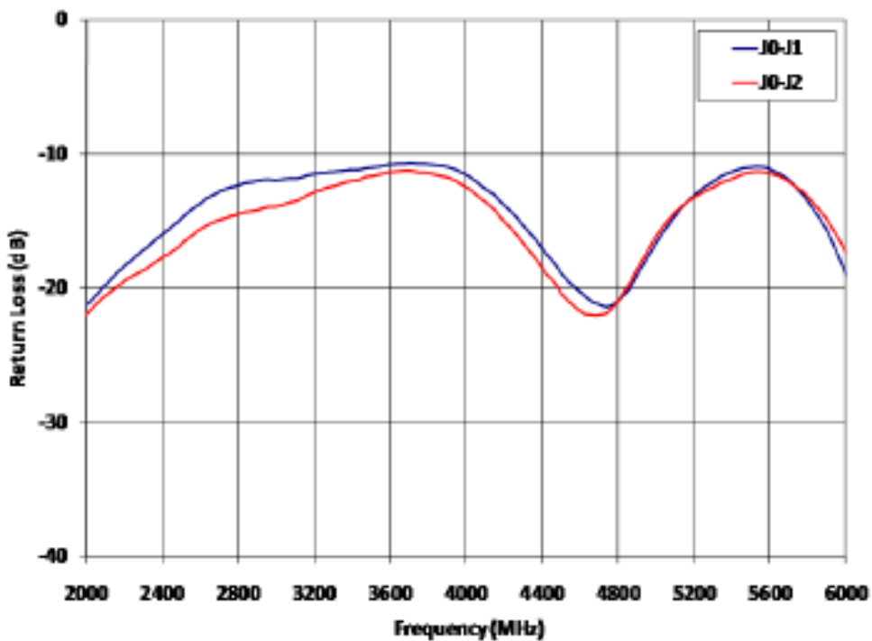
MSW2T-2032-192 Return Loss vs. Frequency
