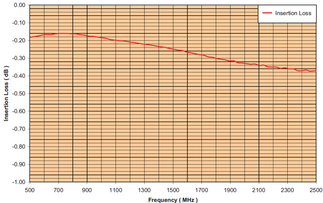
RFLM-501202MC-299 Insertion Loss vs Frequency
