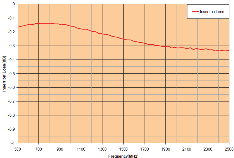
RFLM-501202LC-299 Insertion Loss vs Frequency
