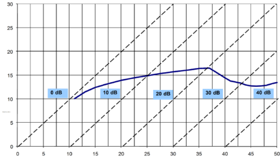
CW Output Power vs. CW Input Power
