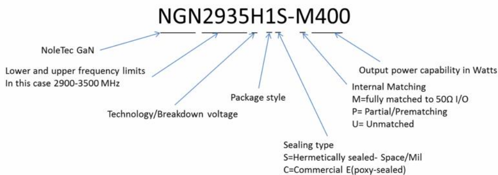
Package style 4
